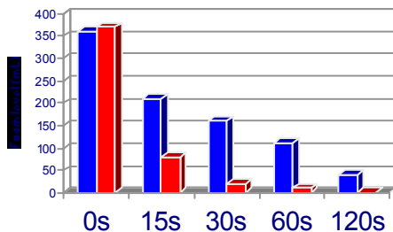
Defoaming ability
